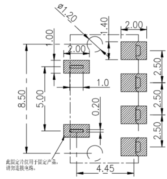
RECOMMENDED PCB LAYOUT TOP VIEW (. XX ± 0.05)
